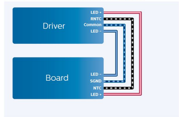
Connection between driver and FF-module
