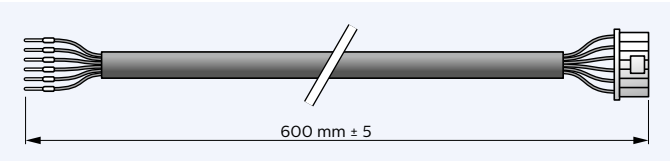
Used cable between driver and LLM-module Cable Fortimo 7 PA to 6 wire – 600 mm (9290 008 03903)
