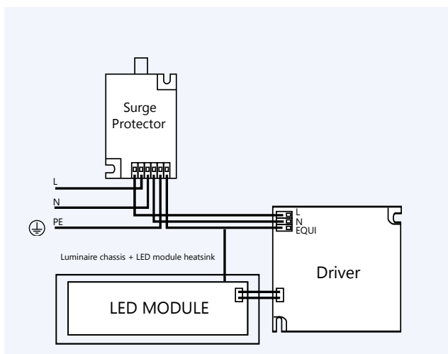
Recommended SPD connection
