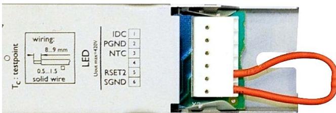
Example of an insulated Rset2 resistor into a non-isolated driver
