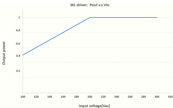
Derating curve of WL LP 100W driver
