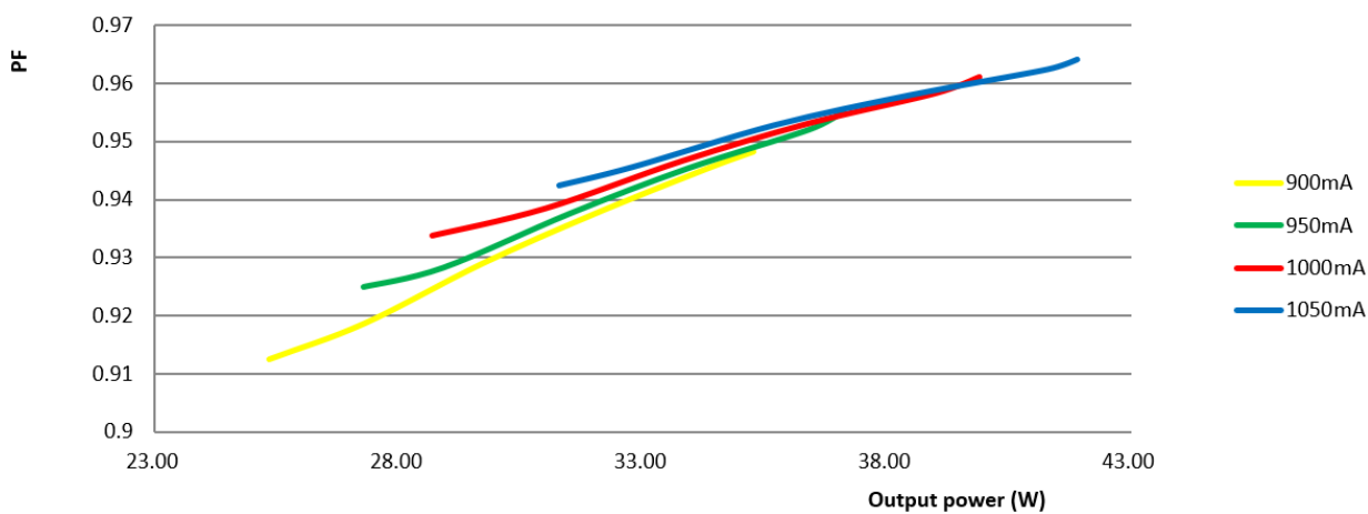
Power factor versus output power
